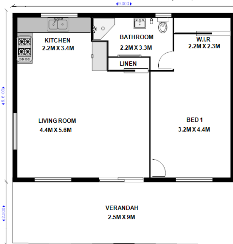
1 Bedroom, 1 Bathroom Ashmore Floor Plan
